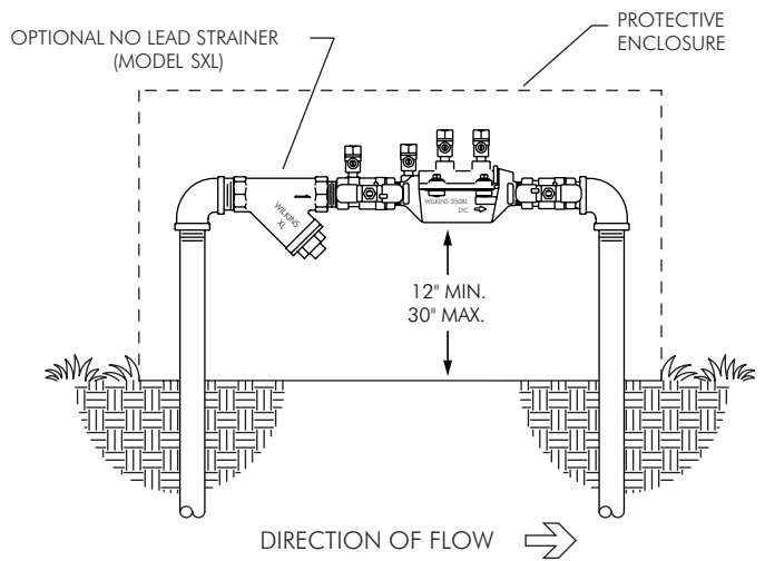
OUTDOOR INSTALLATION
