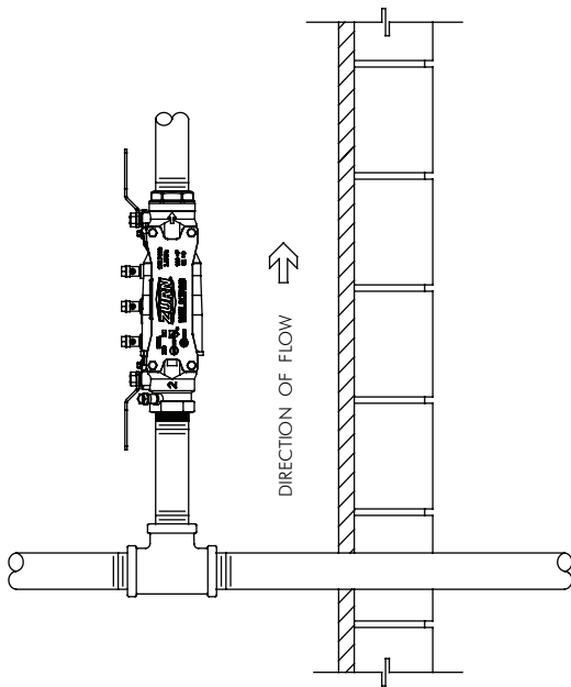
INDOOR INSTALLATION
