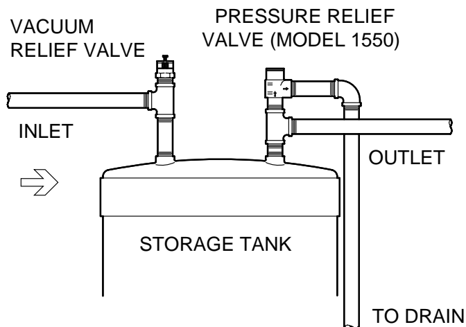
TYPICAL INSTALLATION
