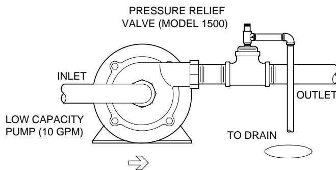
TYPICAL INSTALLATION
