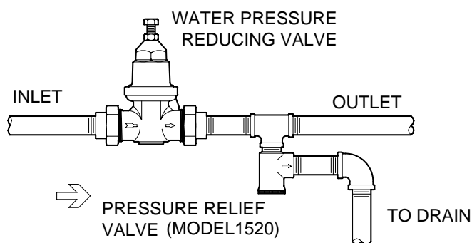
TYPICAL INSTALLATION
