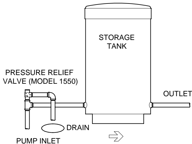
TYPICAL INSTALLATION
