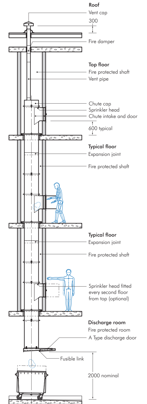
Linen Chute. A Type discharge
